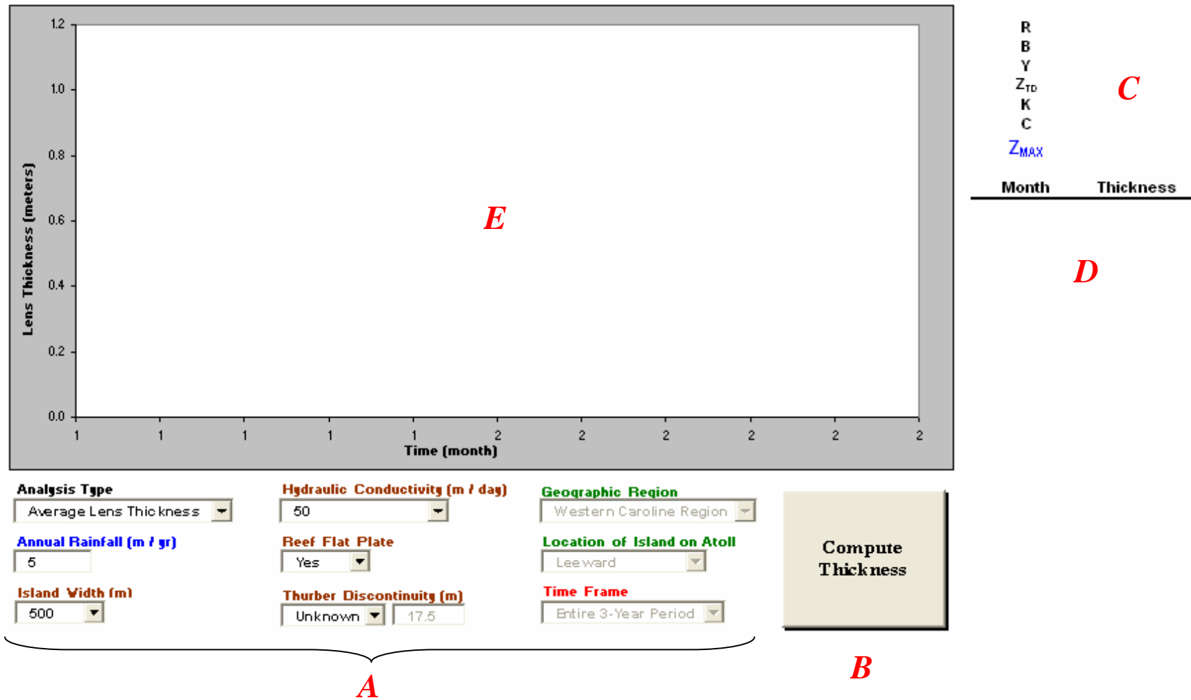
Figure 12. User Interface for the atoll freshwater lens tool spreadsheet. Section A allows the user to enter island attributes, B runs the program which computes the lens thickness, C outputs the algebraic model parameter values calculated from the island attributes, D outputs the thickness of the lens through time, and E displays the resulting curve.
