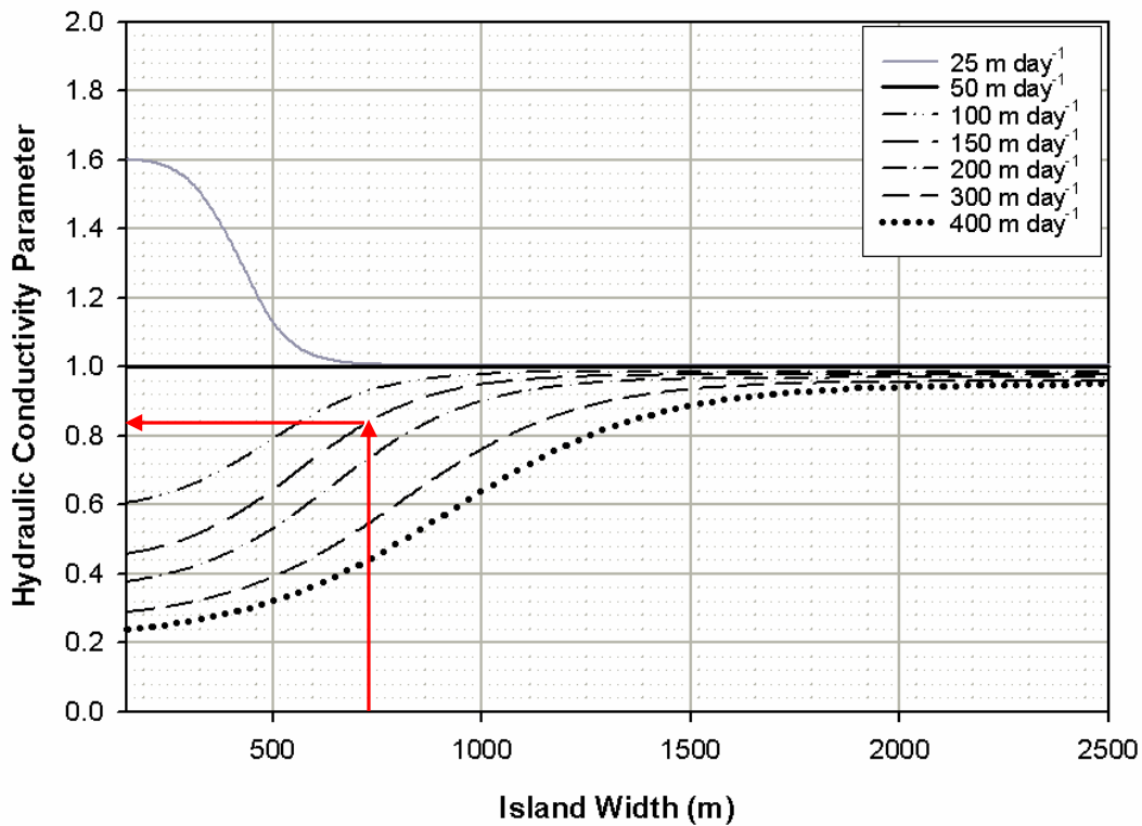
Figure 8. Curves for determining the value of the K factor
