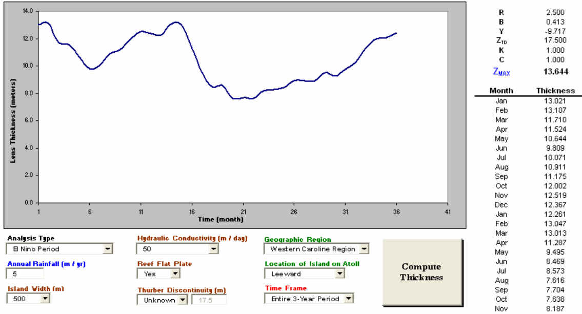
Figure 16. User interface and results for an El Niño Period analysis
