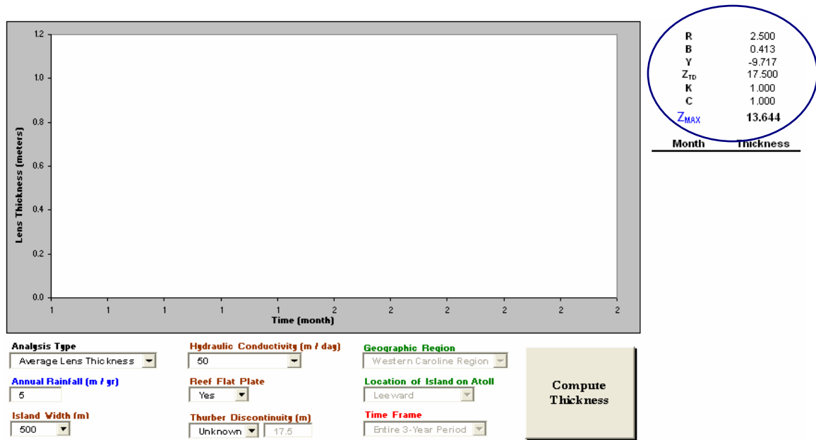
Figure 14. User interface and results for an Average Lens Thickness analysis. The calculated parameter values for the atoll freshwater lens algebraic model are circled in blue.
