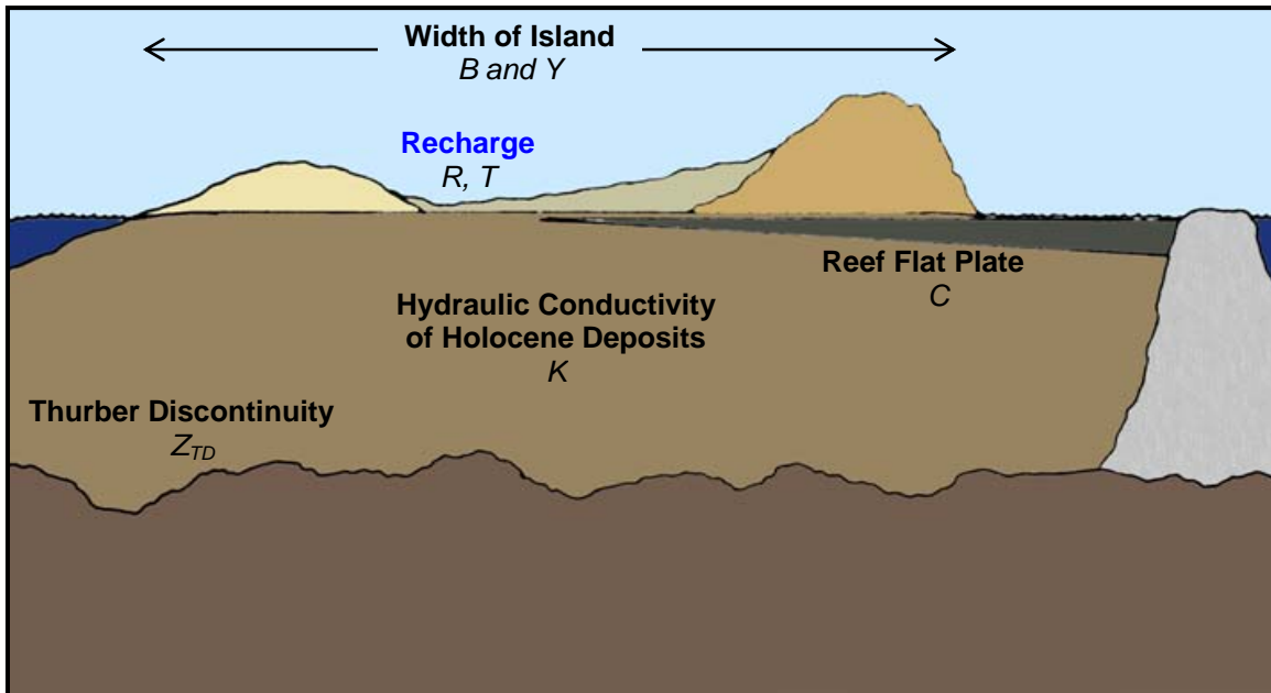
Figure 6. Climatic and geologic factors included in the Algebraic Model
