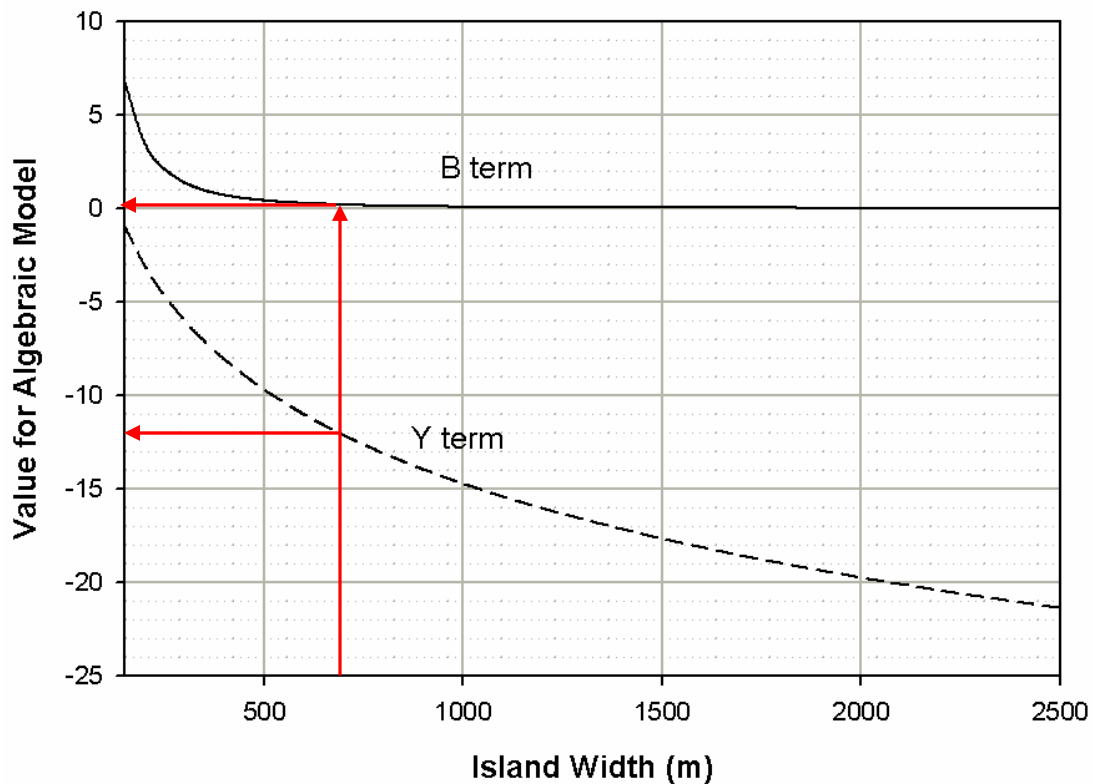
Figure 7. Curves to determine the value of the B and Y parameters. The parameters are dependent upon the width of the island.
