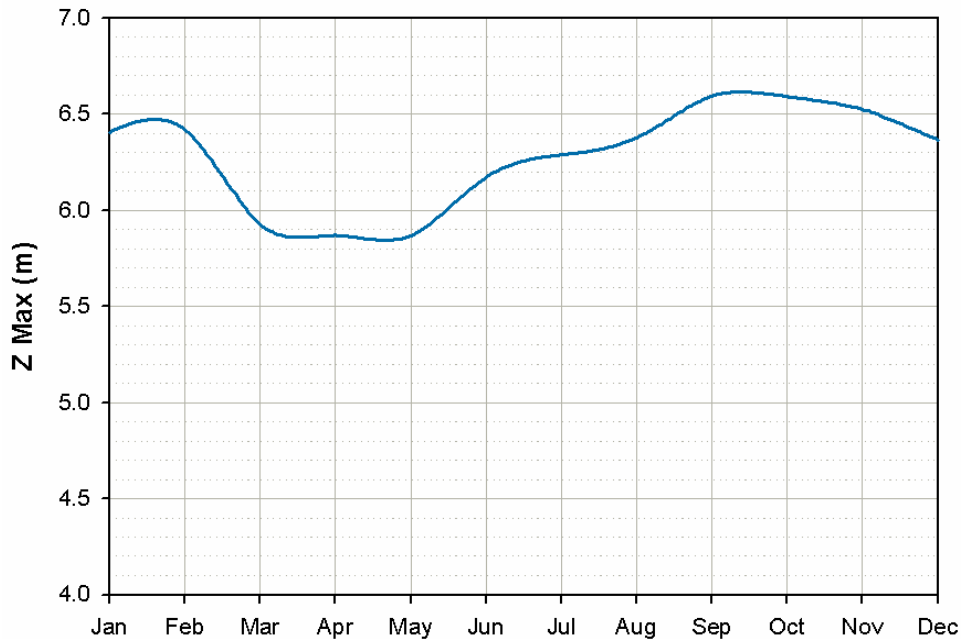
Figure 10. Freshwater lens fluctuation during average seasonal rainfall pattern
