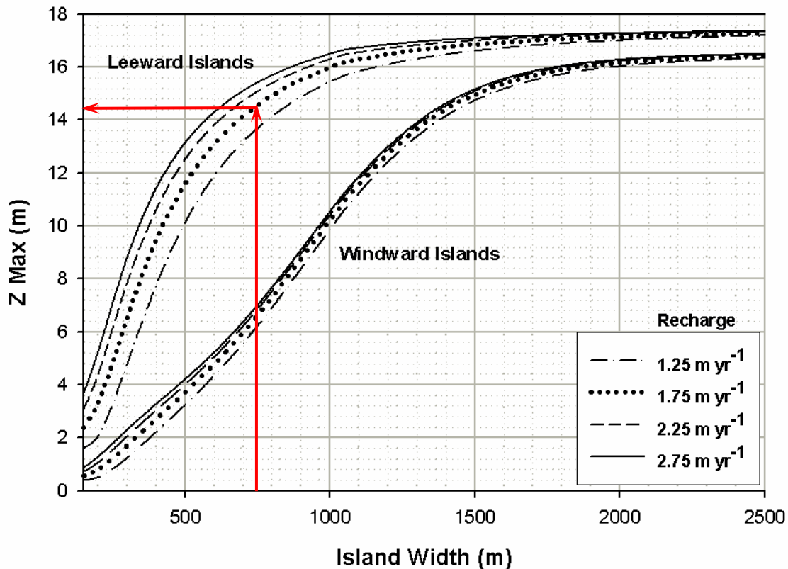
Figure 17. Curves to calculate the thickness of the freshwater lens
