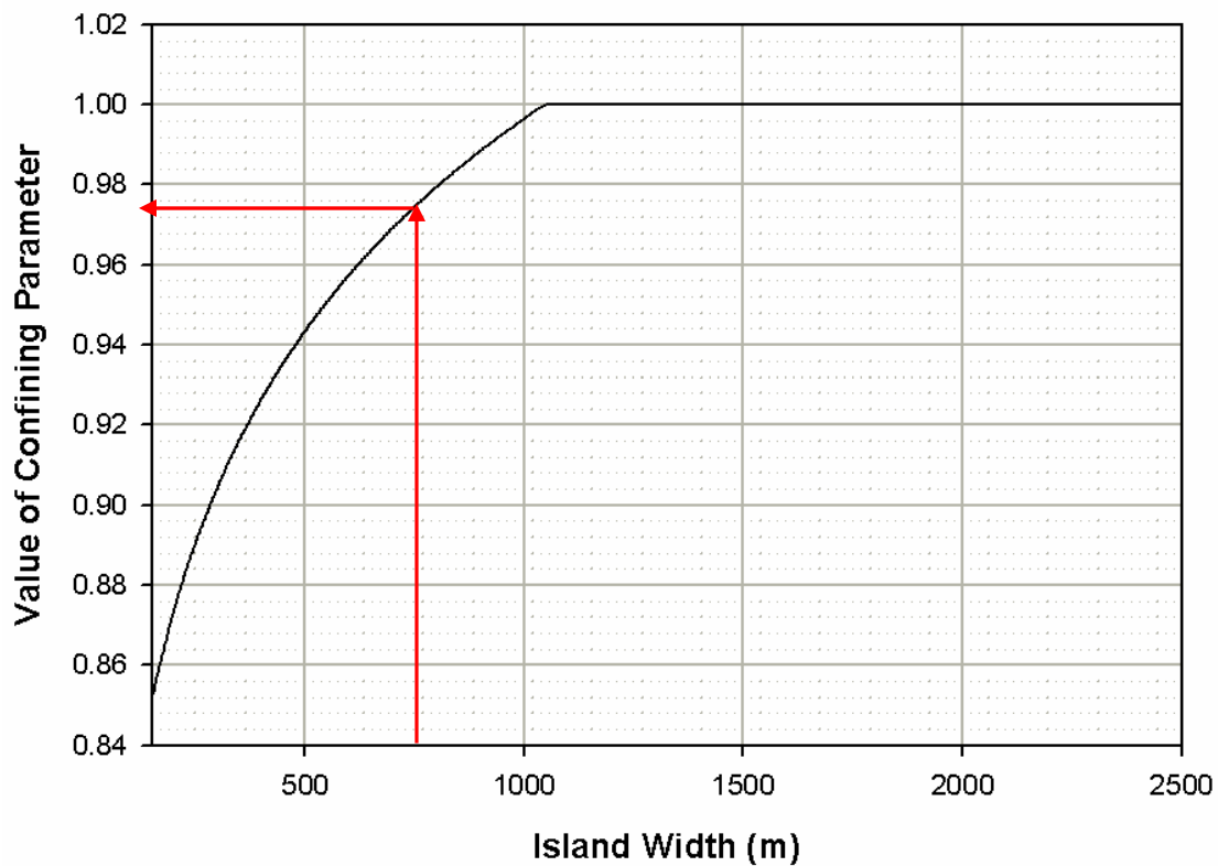
Figure 9. Curve for determining the value for the RFP factor
